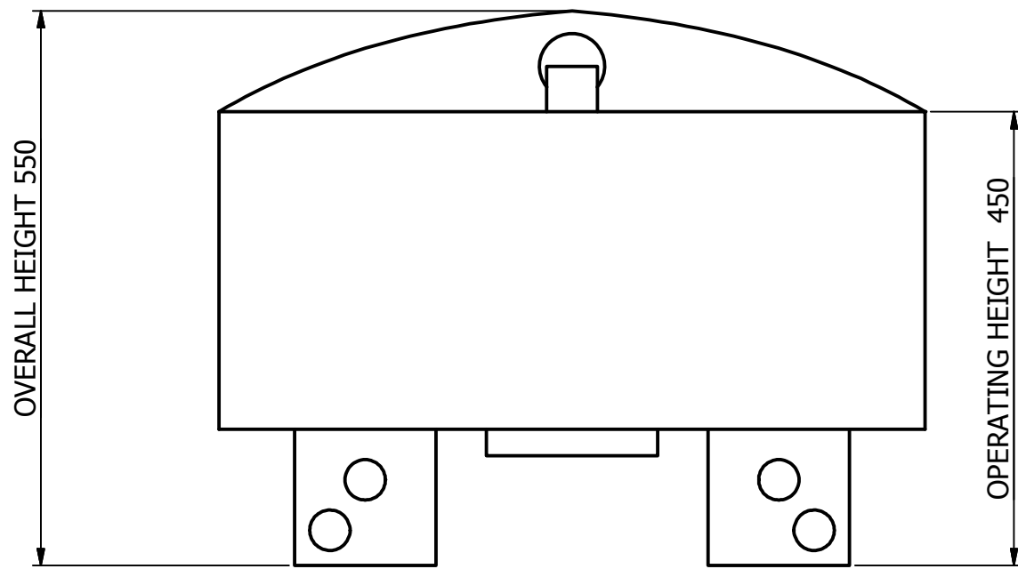
ELEVATION VIEW
