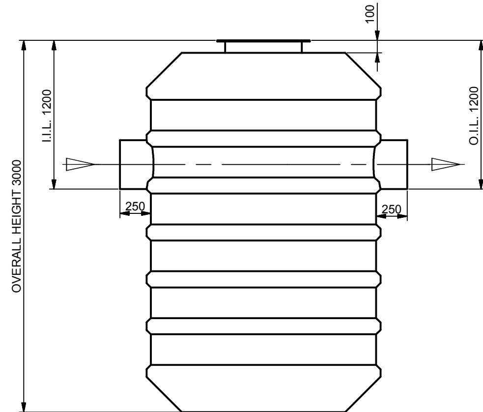
ELEVATION VIEW
