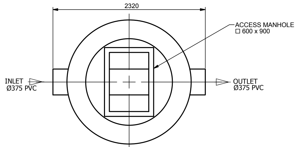
PLAN VIEW
